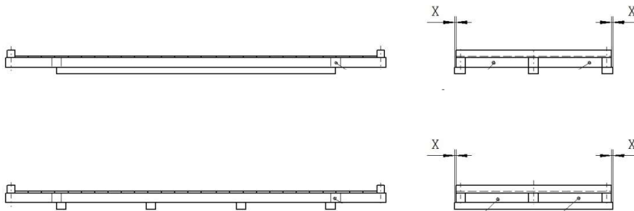
Figure 12: Skid protrusion X
