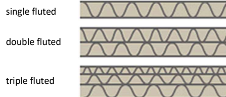
Figure 9: Composition of corrugated cardboard
