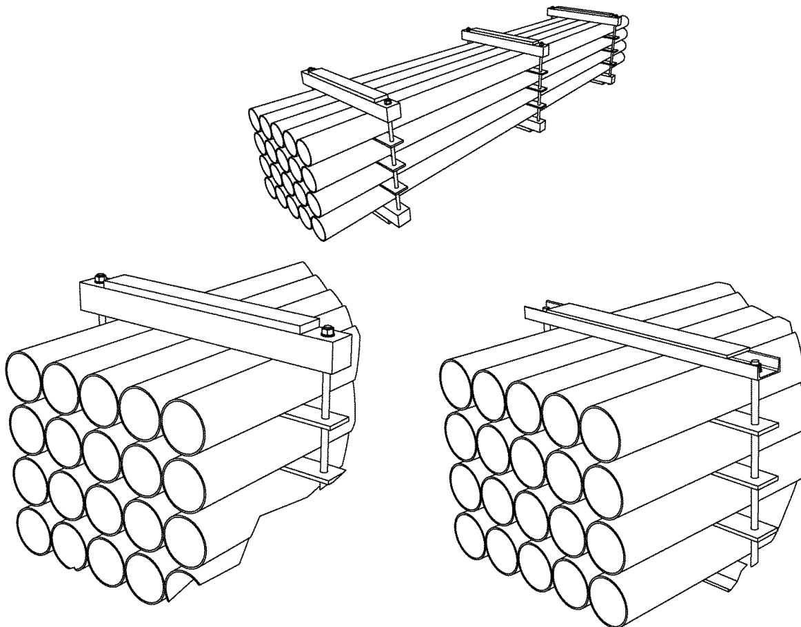
Figure 10: Bundles having clamps made of squared timbers or sectional steel
