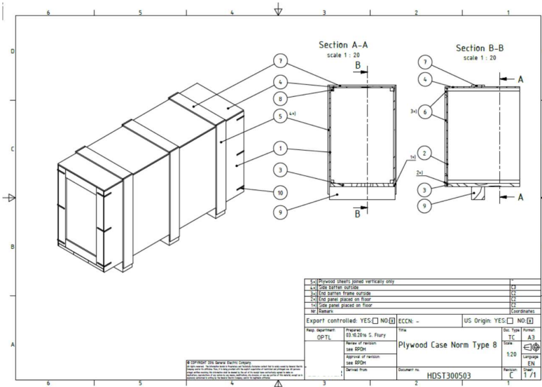
Figure 6: Plywood box type 8
