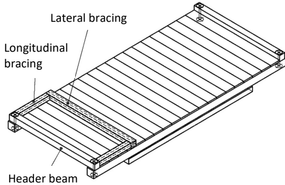
Figure 15: Structure of bracing without direct bolting
