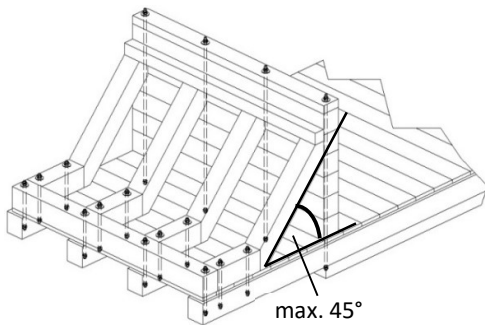
Figure 18: Maximum angle of supporting timbers
