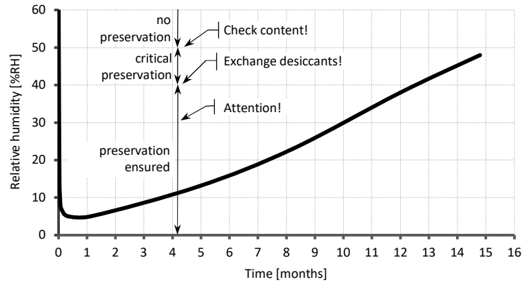
Diagram 1: Relative humidity over time within the foil packaging
