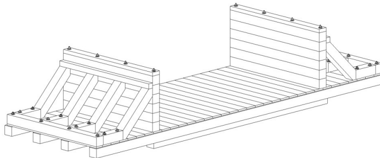
Figure 17: Bottom design with supports and supporting beams
