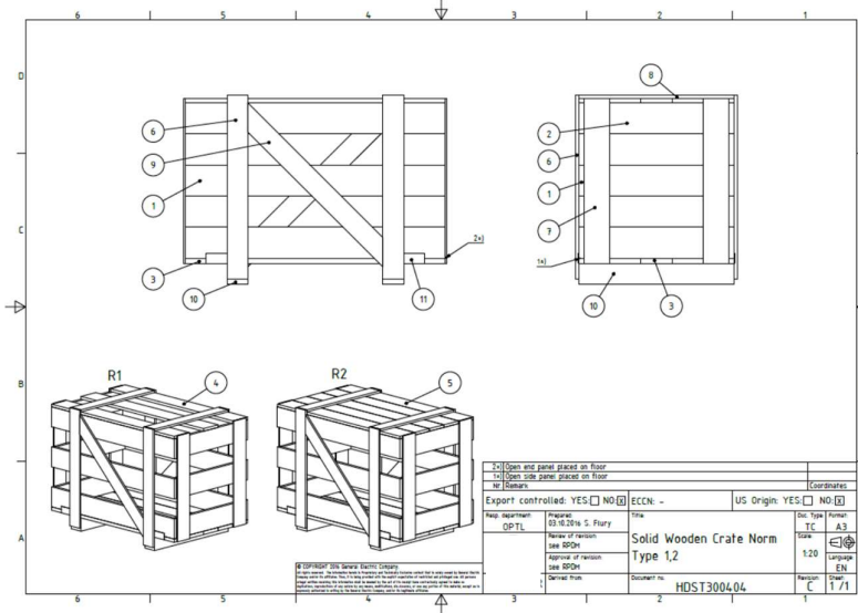
Figure 7: Solid wooden crate type 1 and 2
