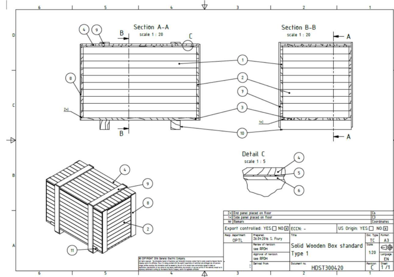
Figure 1: Solid wooden box type 1
