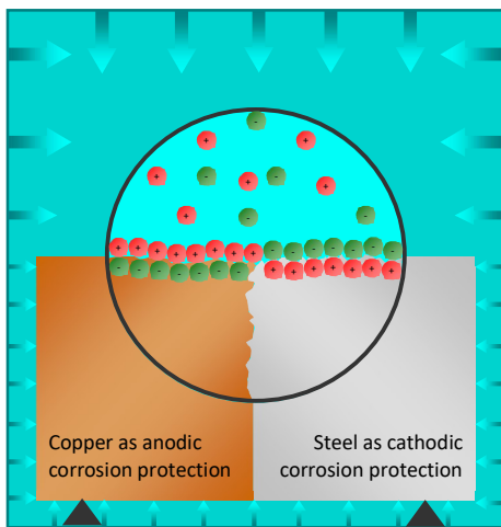
Figure 38: Functional principle
