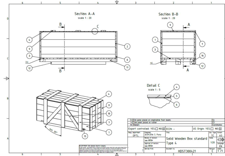
Figure 2: Solid wooden box type 4
