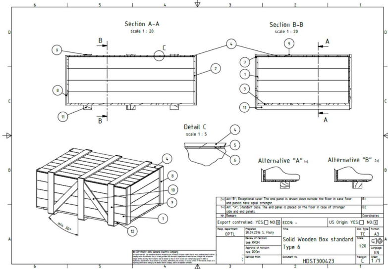
Figure 4: Solid wooden box type 6
