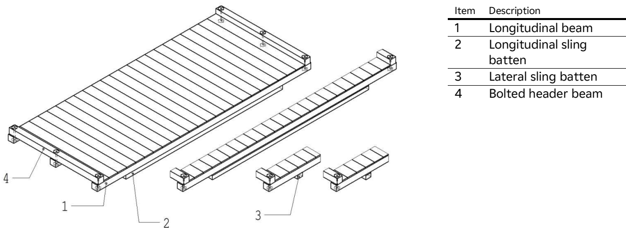
Figure 11: Bottom elements
