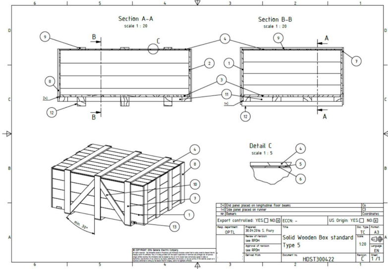
Figure 3: Solid wooden box type 5
