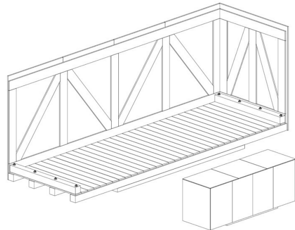
Figure 25: Box cladding made of plywood panels
