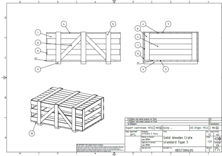
Figure 8: Solid wooden crate type 3
