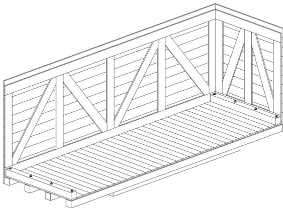
Figure 24: Box with horizontal saw wood boarding
