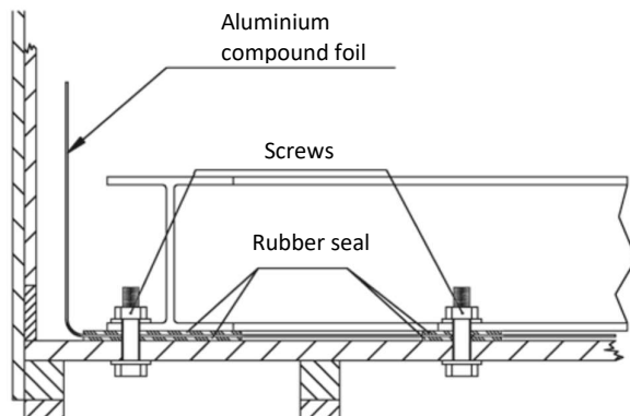
Figure 14: Foil sealing of bolted connections
