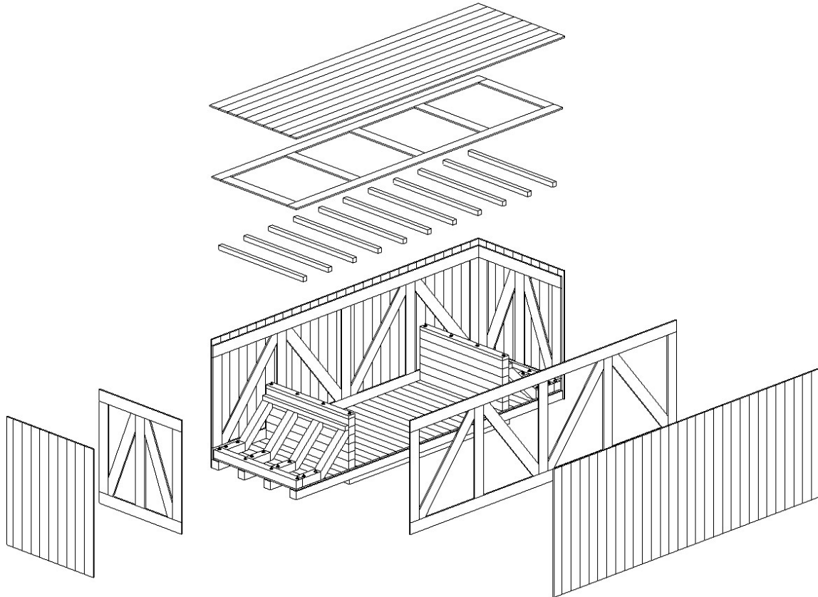
Figure 20: Composition of box walls
